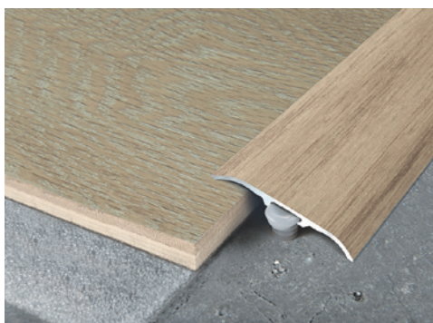
Fixation with adhesive + screw anchor Moderate pedestrian traffic
