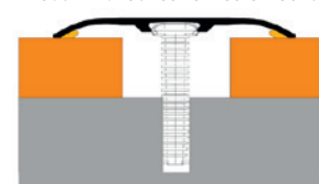
Fixation with adhesive + screw anchor
